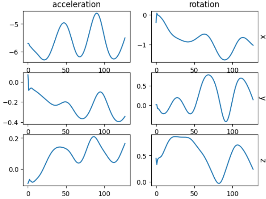
Figure 23: Generated Sequence with simple RNN model
