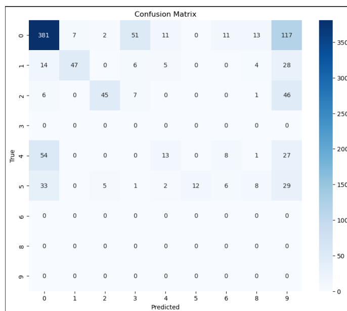
Figure 13: Confusion matrix of best reproduced model (49.75% accuracy)
