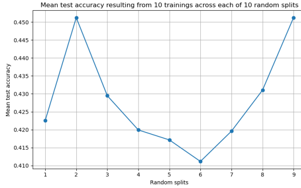
Figure 11: Mean test accuracy of each 10 trainings over each of the 10 random splits
