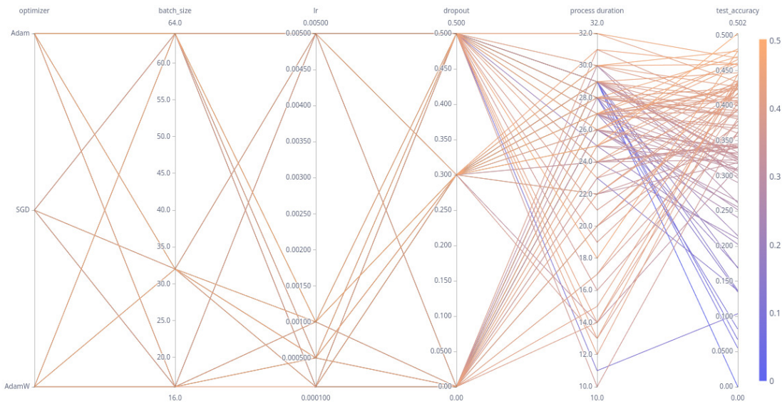
Figure 10: Parallel coordinate plot for the experiment with the 2D CNN
