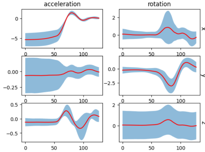
Figure 27: The deviation plot over time for the data in test.pkl . The red graph is the mean \mu_t over time t . The blue area is the space between \mu_t - \sigma_t and \mu_t + \sigma_t .
