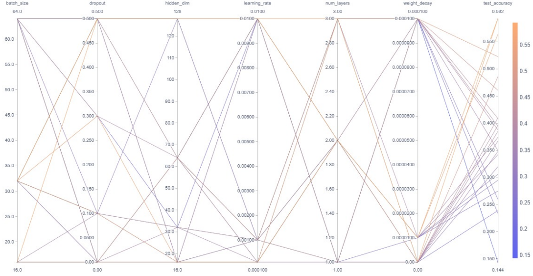
Figure 14: All 100 randomly selected training runs without random splitting or early stopping from high test accuracy to low test accuracy
