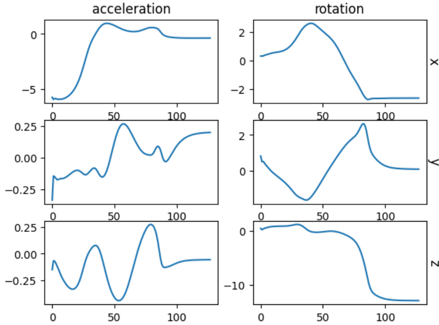
Figure 25: Generated Sequence with flatness-rewarding generator
