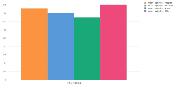
Figure 5: Test data evaluation Accuracy, for each optimizer
