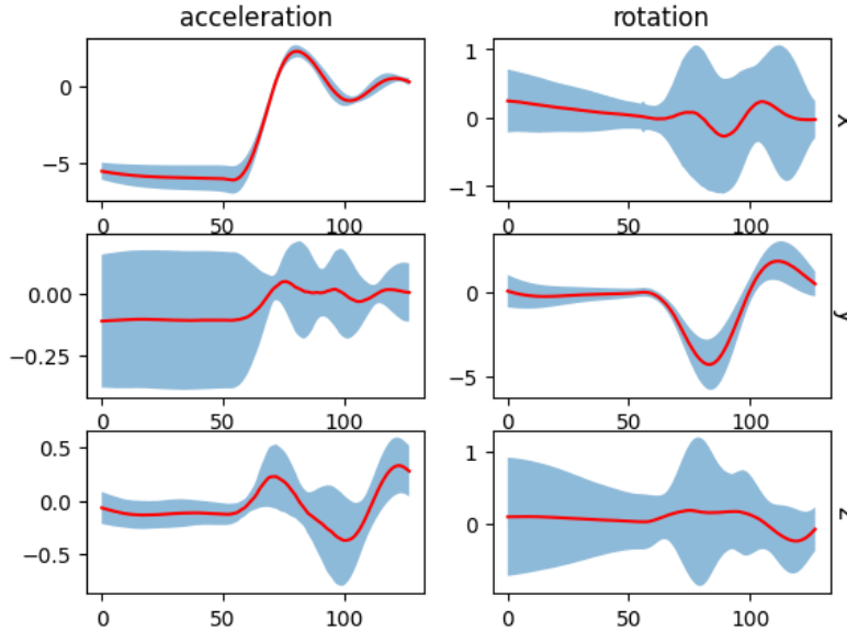
Figure 20: The deviation plot over time. The red graph is the mean \mu_t over time t . The blue area is the space between \mu_t - \sigma_t and \mu_t + \sigma_t .
