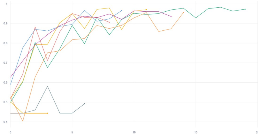
Figure 18: Validation accuracy across 10 random splits over 20 epochs
